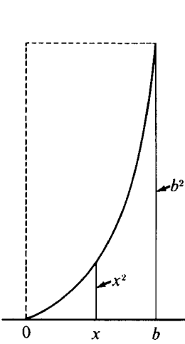
FIGURE I.3 A parabolic segment.
